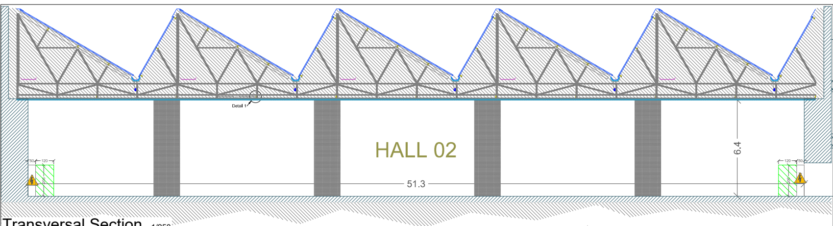
Transversal Section 1/250
