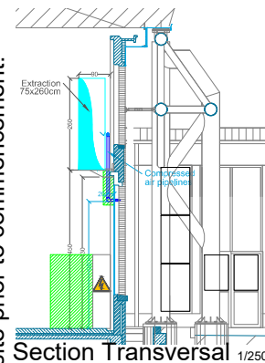
Section Transversal 1/250
