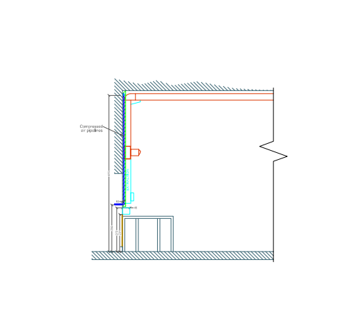
Transversal Section 1/200
